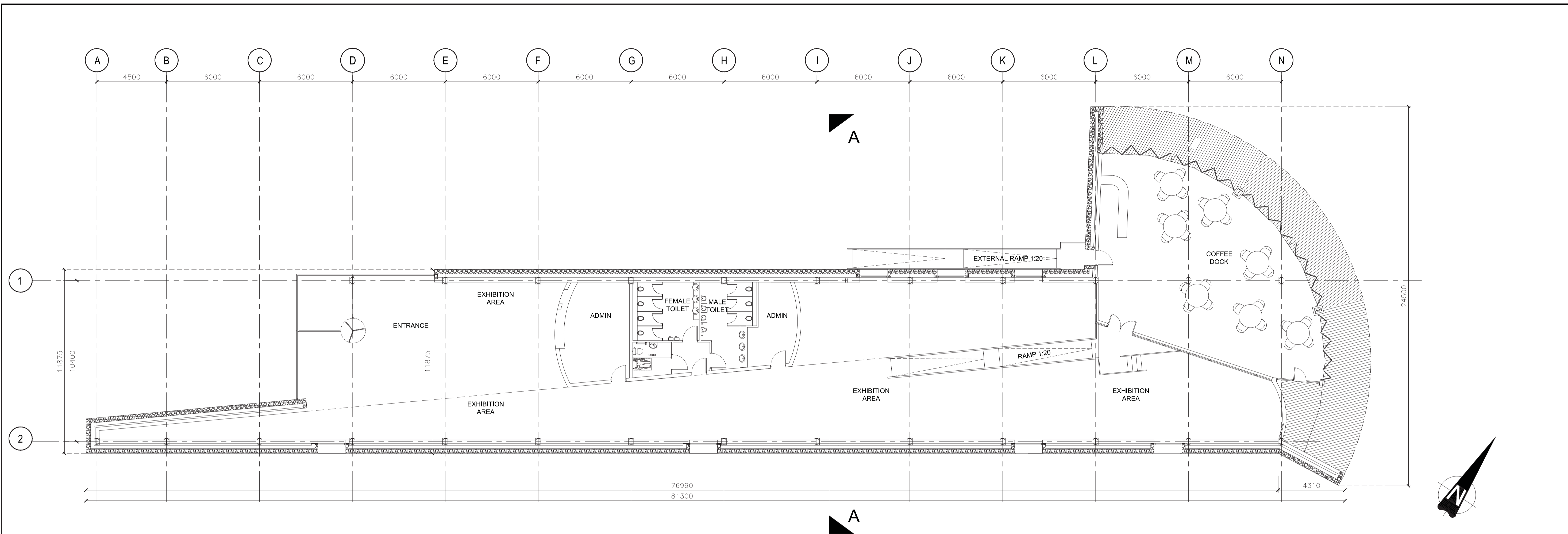
GROUND FLOOR PLAN SCALE 1:125
