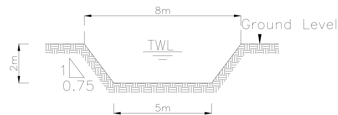
Section 1 - 1
